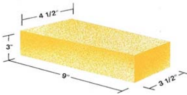
9 Inch No. 2 Key 9 x (4 1/2 - 3 1/2) x 3
