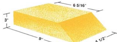
(9 - 6 5/16) x 4 1/2 x 3
