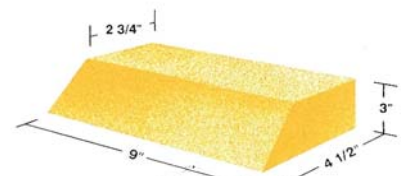
9 Inch - 60° Side Skew 9 x (4 1/2 - 2 3/4) x 3
